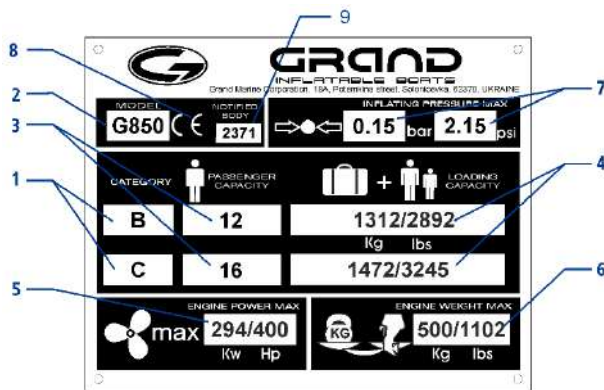
Fig.15. Builder's plate.
