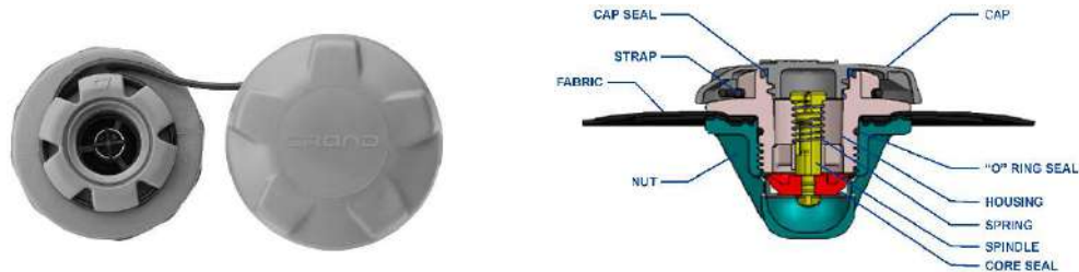
Fig 17. Inflation valve.
